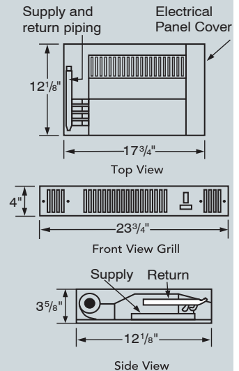
WH III 9000 Kickspace Heater
