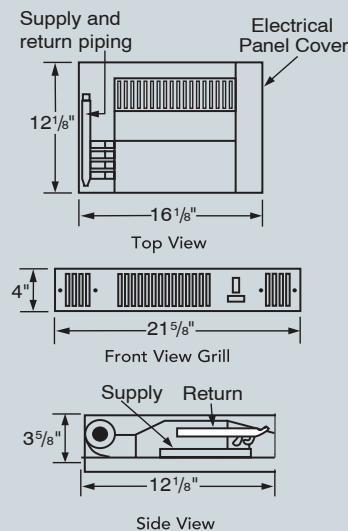
WH III 7000 Kickspace Heater
