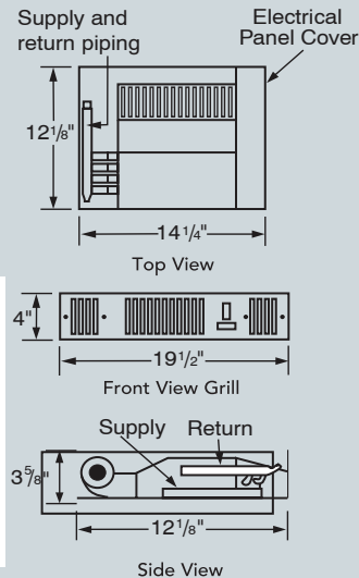
WH III 5000 Kickspace Heater
